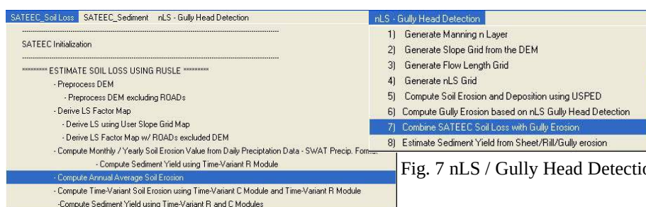
Fig. 6 SATEEC_Soil Loss
